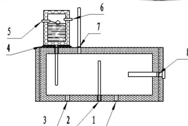
1. Sensor hole 2. Water outlet 3. Drain outlet 4. Rubber blanket 5. Water inlet 6. Air outlet 7. Air out let 8. Electrical heating
