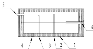
1. Water outlet 2. Air vent 3. Over flow vent 4. Water inlet 5. Sensor hole 6. Electrical element
